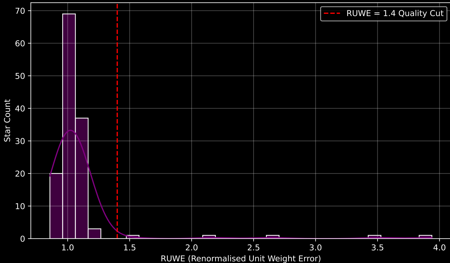
GAPOGEE DR17 Field [Sgr_faint] RUWE Distribution (n= 134)
