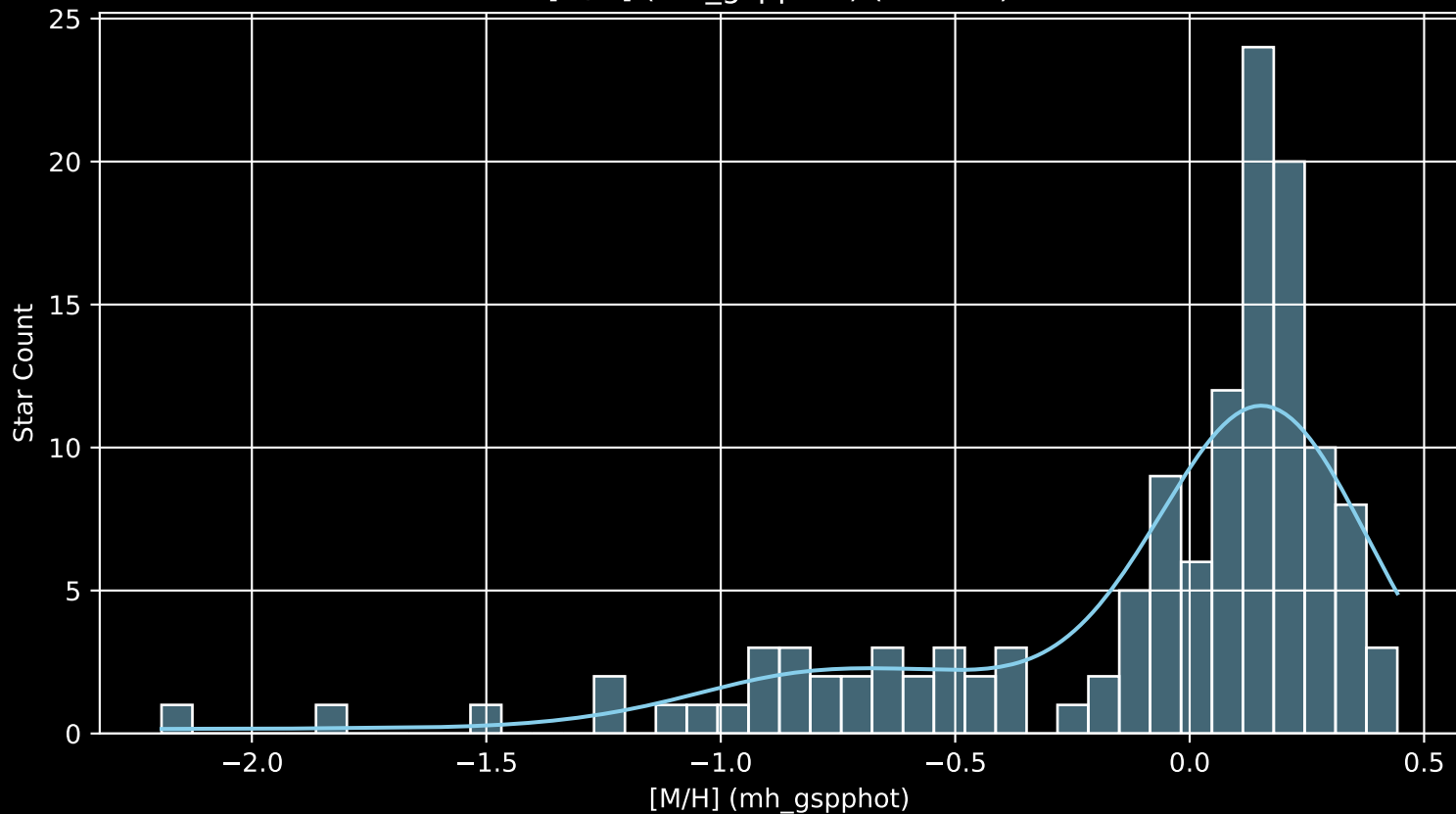
APOGEE DR17 Field: [Sgr_faint [M/H] (mh_gspphot) (n= 131)
