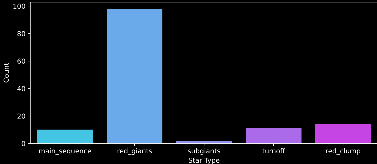
APOGEE DR17 Field: [Sgr_faint] Count plot of Star Type
