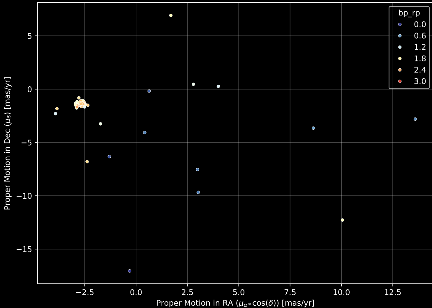
APOGEE DR17 Field: [Sgr_faint] Proper Motion Diagram (n= 135)
