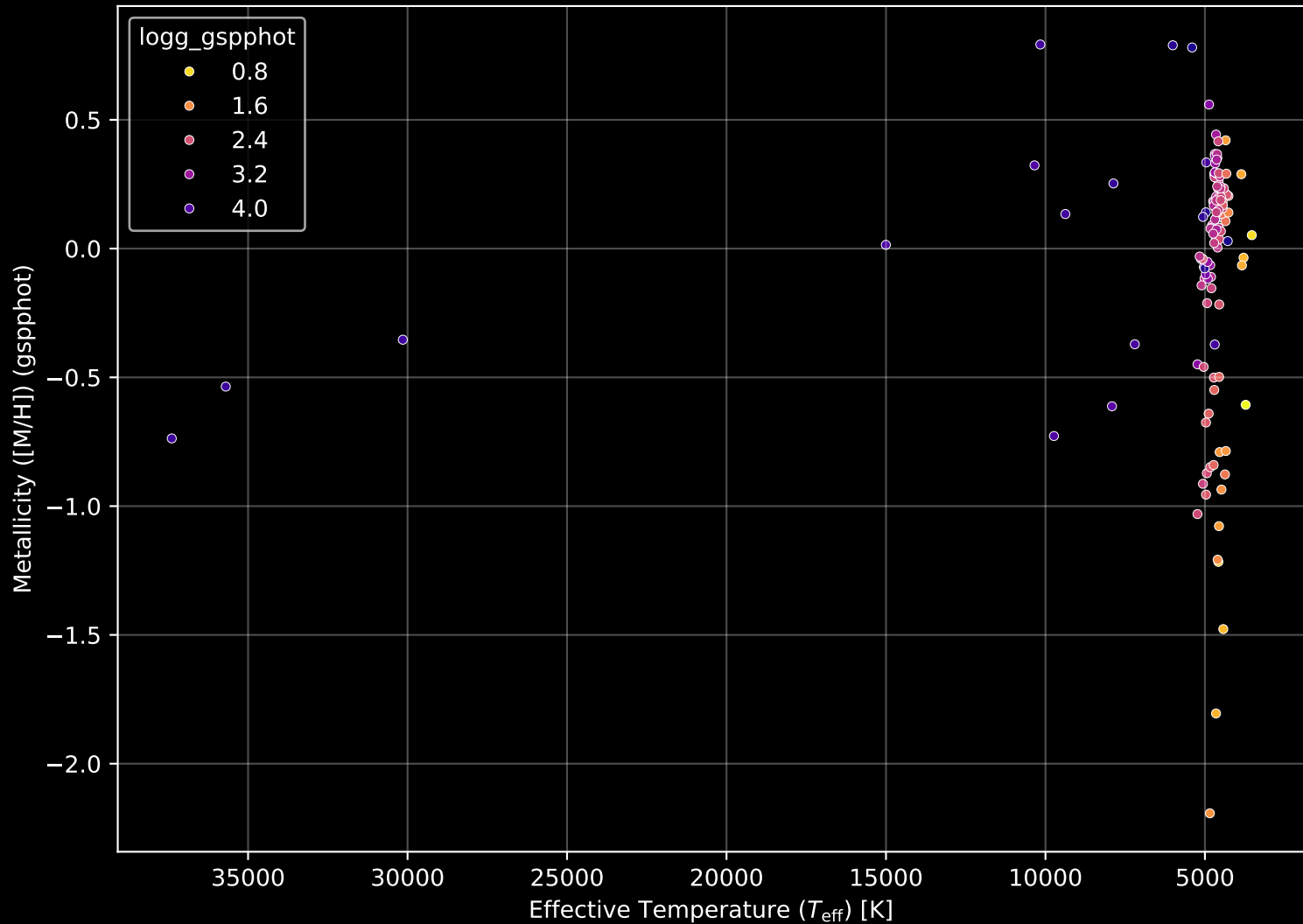
APOGEE DR17 Field: [Sgr_faint] Stellar Population Parameters (n= 135)
