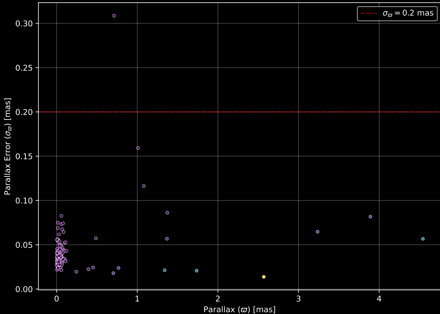
APOGEE DR17 Field: [Sgr_faint] Parallax Quality (n= 135)
