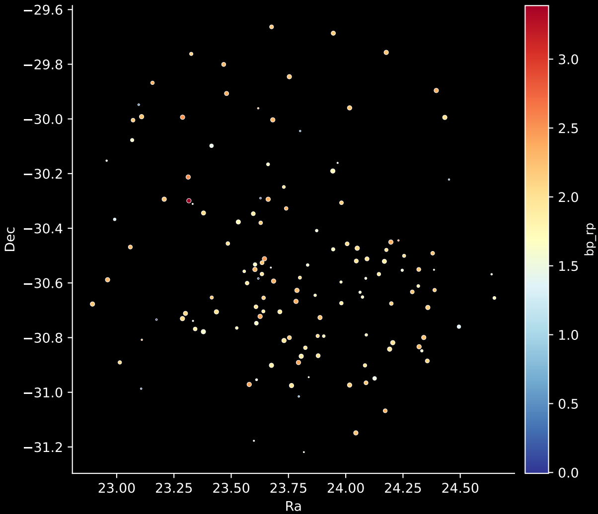
APOGEE DR17 Field: [Sgr_faint] Stars: 135
